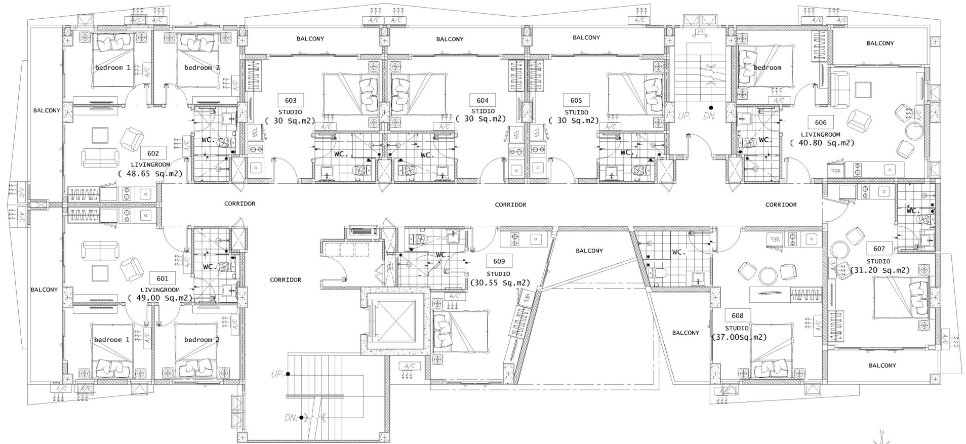
FLOOR PLAN-6
