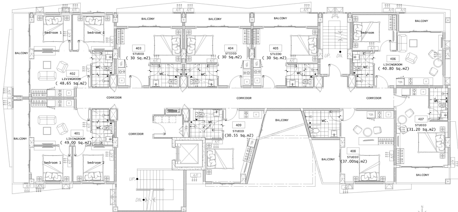
FLOOR PLAN-4
